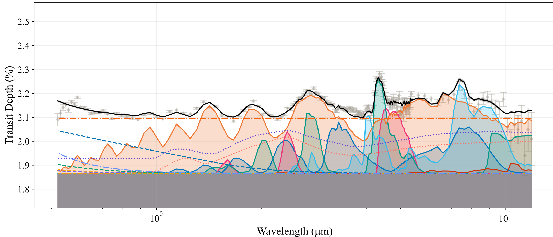
PRISM + MIRI, SO2, Isothermal
